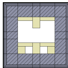
q (1/2)
