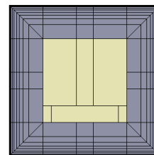
r (1/2)
