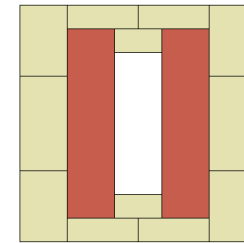
o (1/2)
